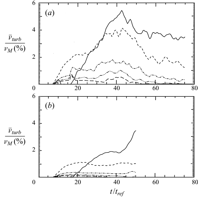
FIGURE 8. Temporal evolution of the ratio \bar{\nu}_{turb}/\nu_M for (a) Re = 5 \cdot 10^4 and (b) Re = 3 \cdot 10^4 . The curves are averages over horizontal planes of constant \eta = 0.35 (—), 0.39 (---), 0.42 (- · - · -), 0.45 (- · · - · · -), 0.47 (— — —).
