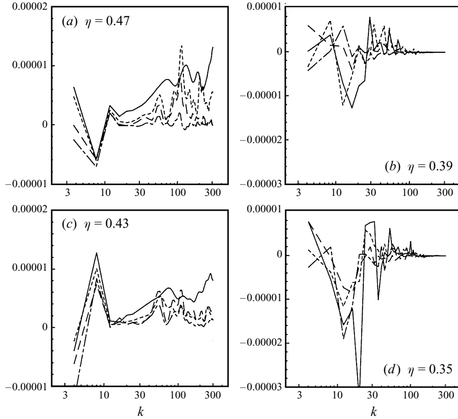
FIGURE 13. Co-spectra of the vertical heat flux \Phi_{w'\theta'}(k) in an early (a, c) and a late period (b, d) of wave breaking. As in figure 9, the individual curves are averages over planes \eta = \text{const} . The lines are for different times: —: 16.5 (a, c), 44 (b, d); - - - - : 17 (a, c), 50 (b, d); - · - · - : 17.5 (a, c), 56 (b, d); · · · · : 18 (a, c), 62 (b, d).
