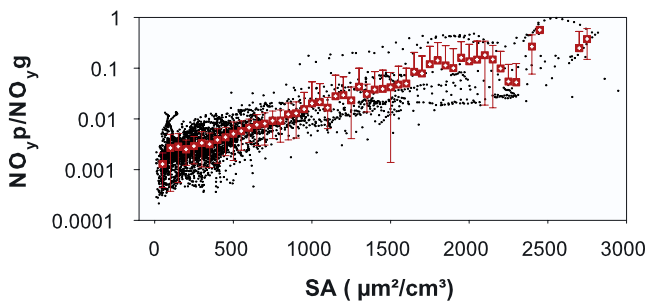
Figure 5. \text{PNO}_y/\text{NO}_{y,\text{gas}} over SA. The ratios are plotted for temperatures and partial pressures within the 25 and 75 percentiles around the respective median values of 226.8 K and 1.37 \times 10^{-8} hPa, respectively. The 1-s data of the ratio are given along with means and standard deviations. The 1-s values have been averaged over SA intervals of 50 \mu\text{m}^2/\text{cm}^3 .
