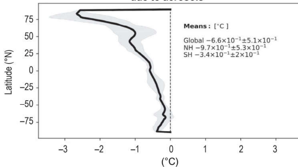
(b) Zonal mean change in surface air temperature due to aerosols
